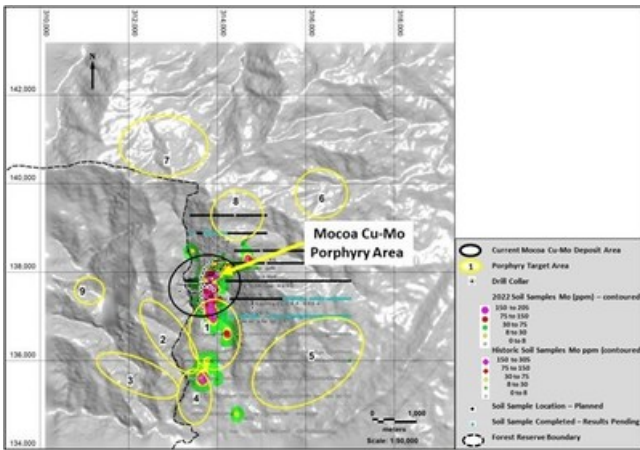
Figure 3: Soil sample geochemical results for Mo and target areas (CNW Group/Libero Copper & Gold Corporation.)
