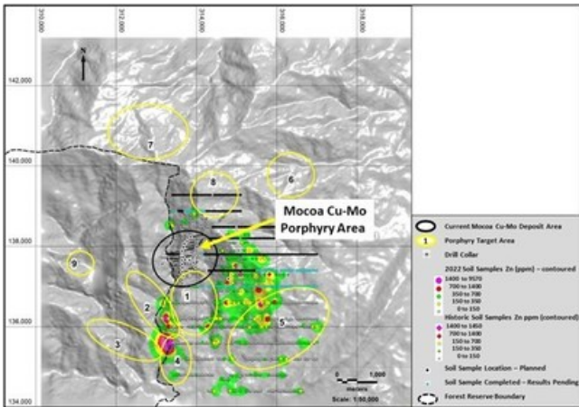
Figure 4: Soil sample geochemical results for Zn and target areas (CNW Group/Libero Copper & Gold Corporation.)
