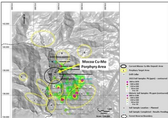
Figure 5: Soil sample geochemical results for Pb and target areas (CNW Group/Libero Copper & Gold Corporation.)
