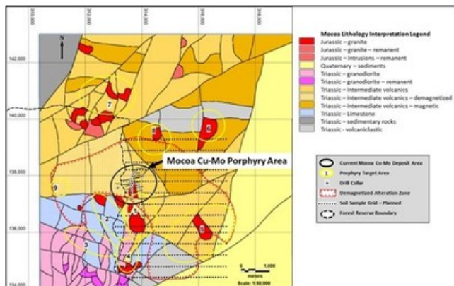
Figure 1: Geological interpretation, Jurassic intrusions (porphyries), 2022 soil sample lines and target areas (CNW Group/Libero Copper & Gold Corporation.)
