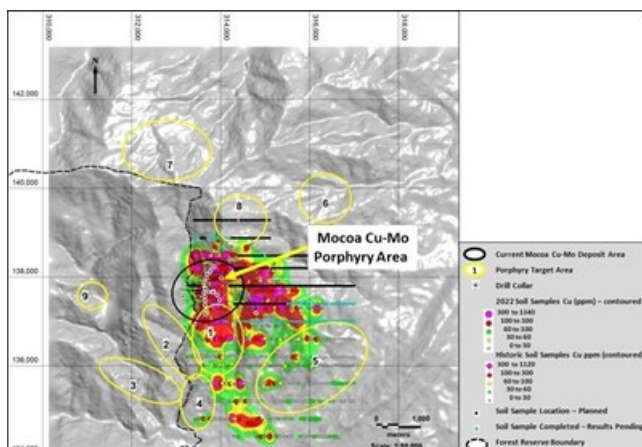
Figure 2: Soil sample geochemical results for Cu and target areas (CNW Group/Libero Copper & Gold Corporation.)
